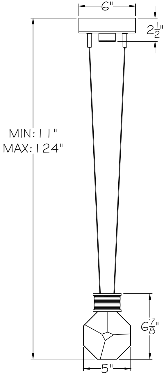
FRONT VIEW
