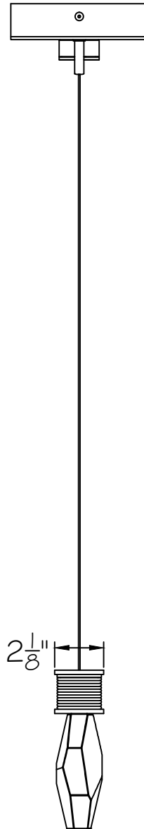
SIDE VIEW
